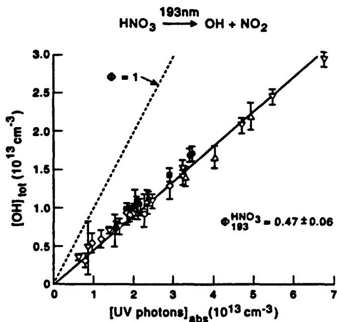
Fig. 7. Sample data plot for determining the quantum yield for OH production from \text{HNO}_3 photolysis at 193 nm.
